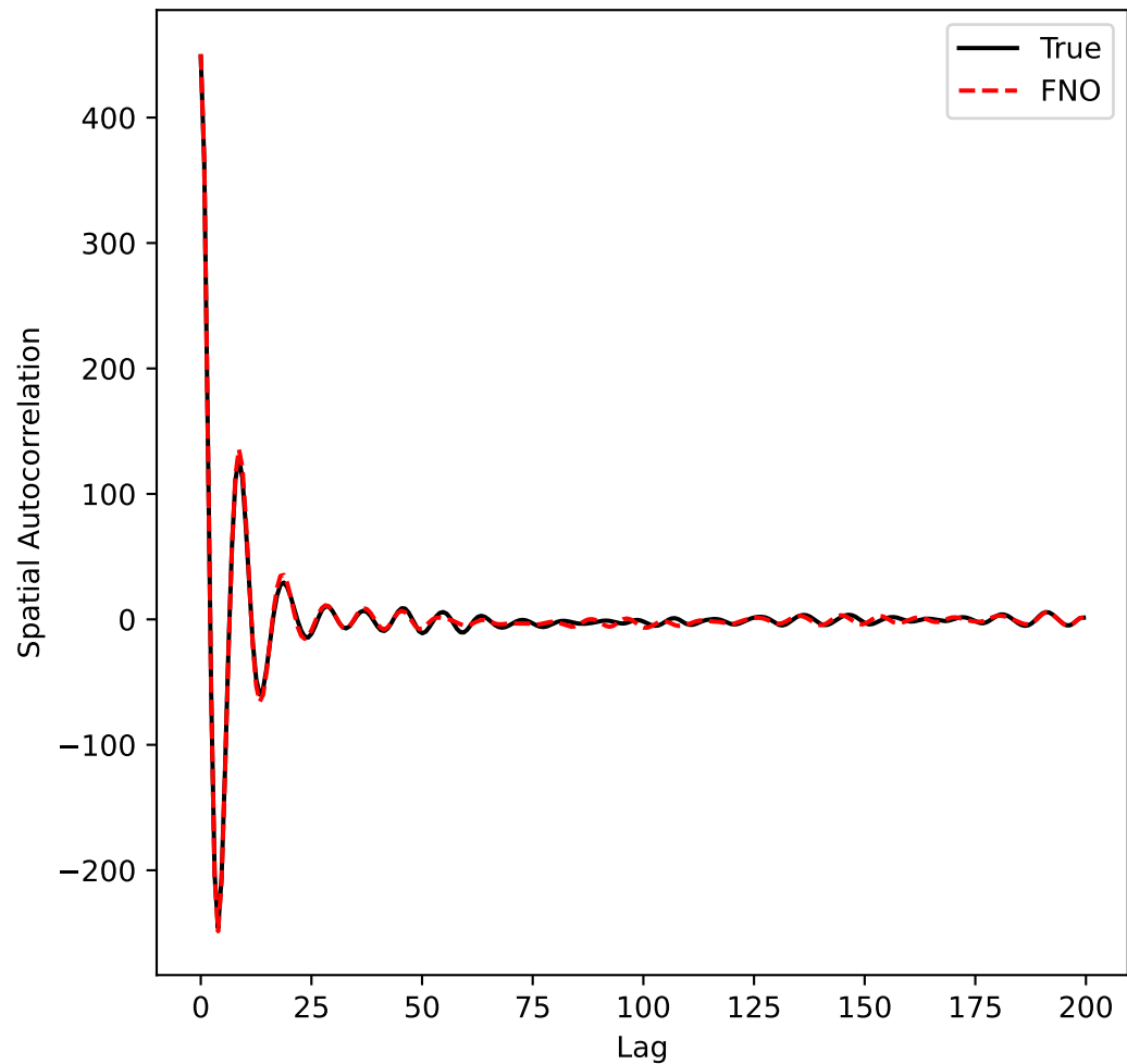
Autocorrelation Comparison with MSE = 6.5
