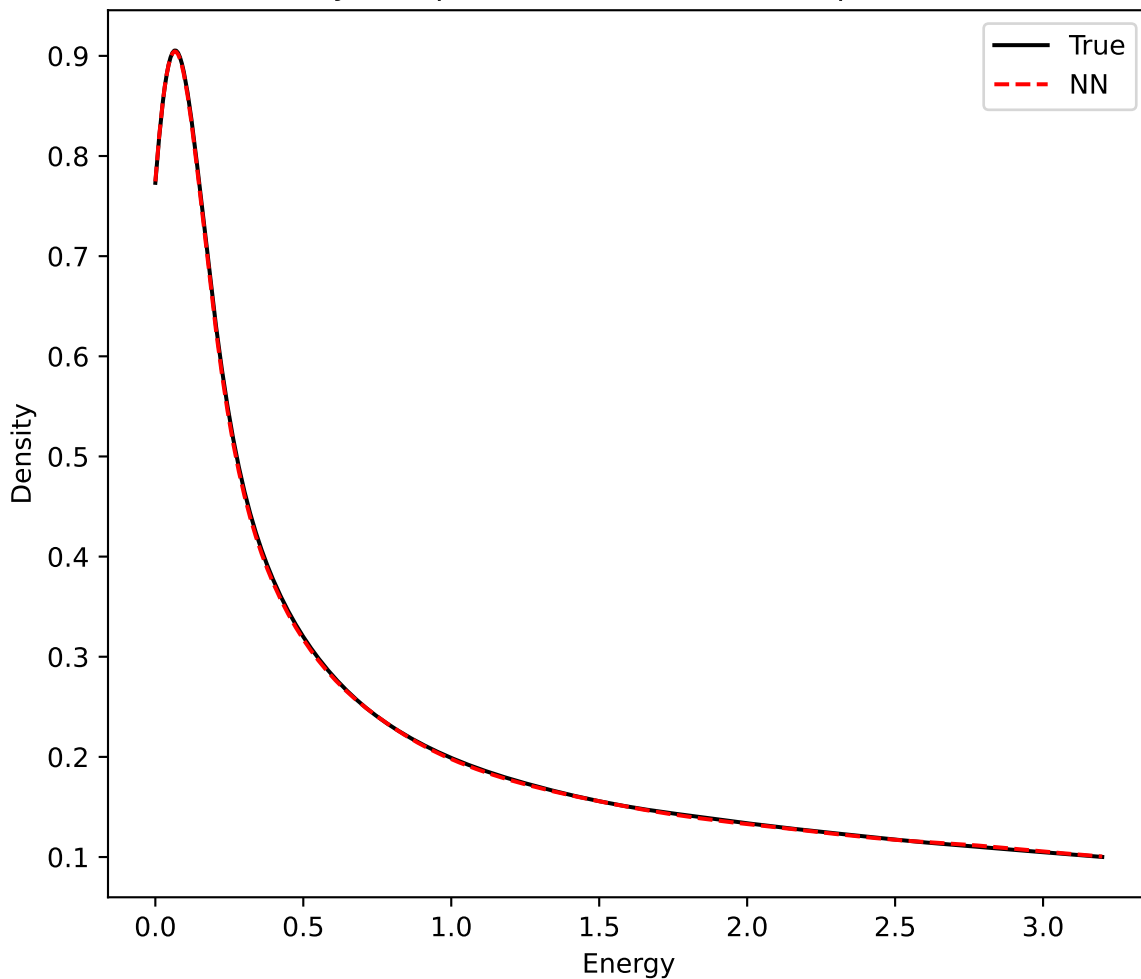
TKE Density Comparison with KS: 0.0028, p-value: 8.6e-11
