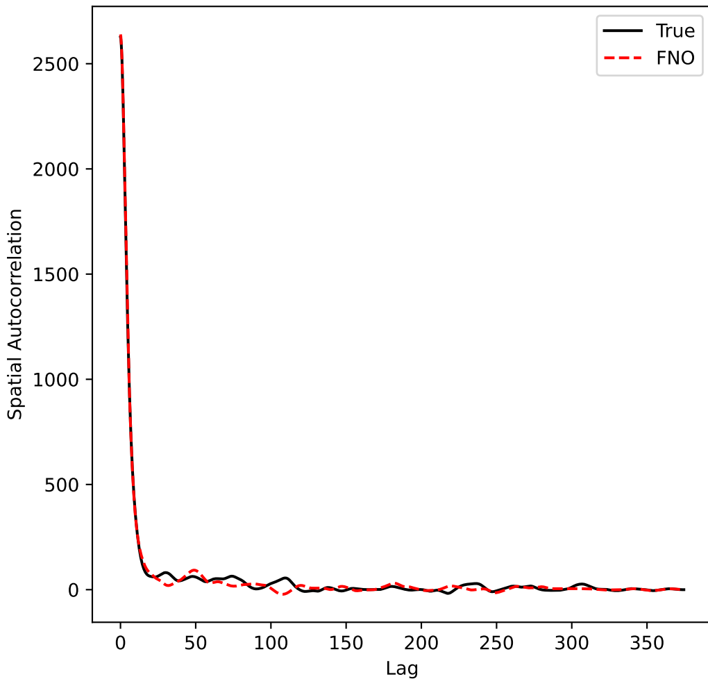
Autocorrelation Comparison with MSE = 3.8e+02
